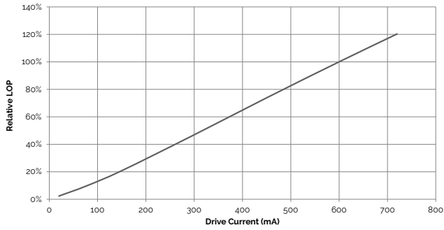
Figure 6: Relative LOP vs. Drive Current, T_c=25^\circ\text{C}
