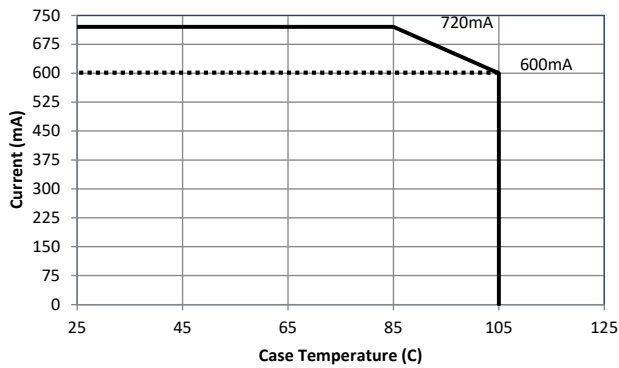
Figure 8: Derating Curve
