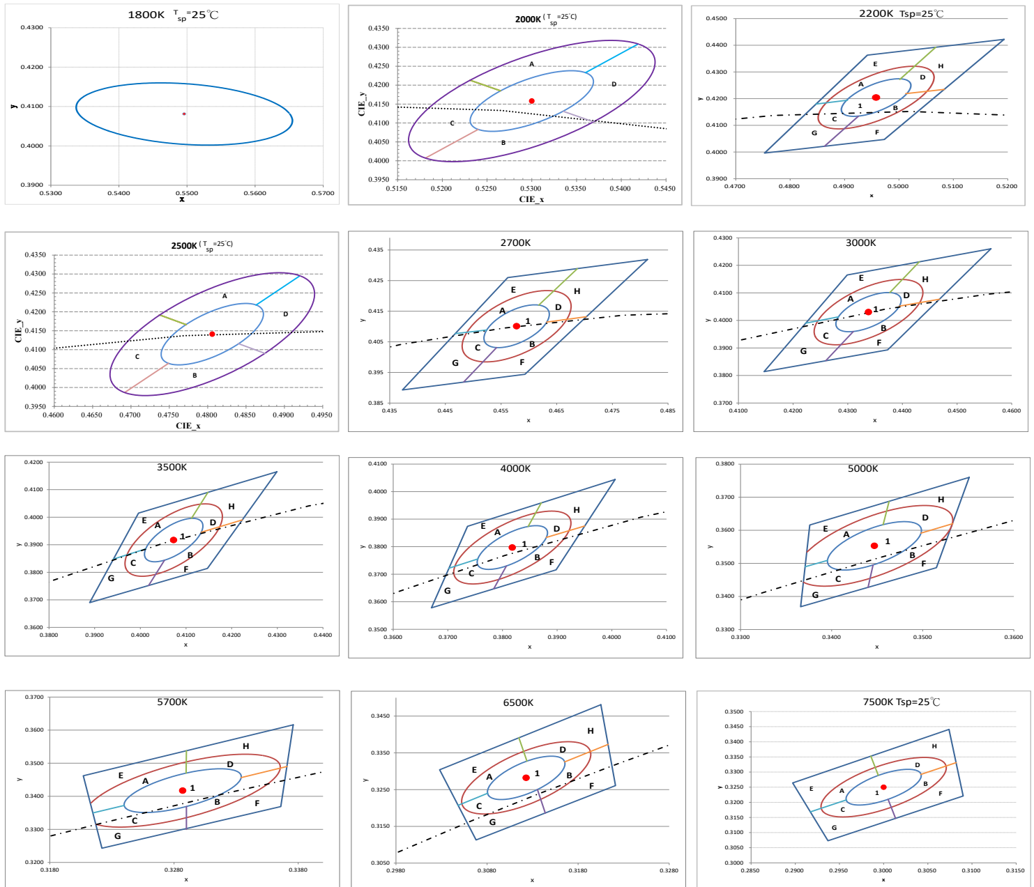
Figure 1: C.I.E. 1931 Chromaticity Diagram (9 Color Bin Structure, Hot-color Targeted at T_{sp}=85^{\circ}\text{C} , 18G / 20G / 22G / 25G / 75G at T_{sp}=25^{\circ}\text{C} )
