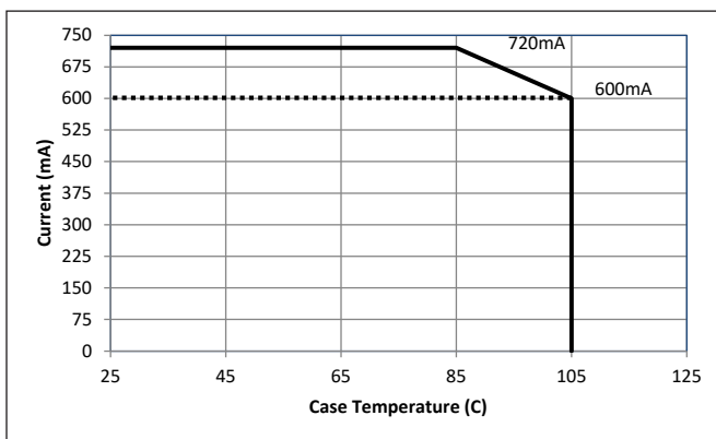
Figure 8: Derating Curve
