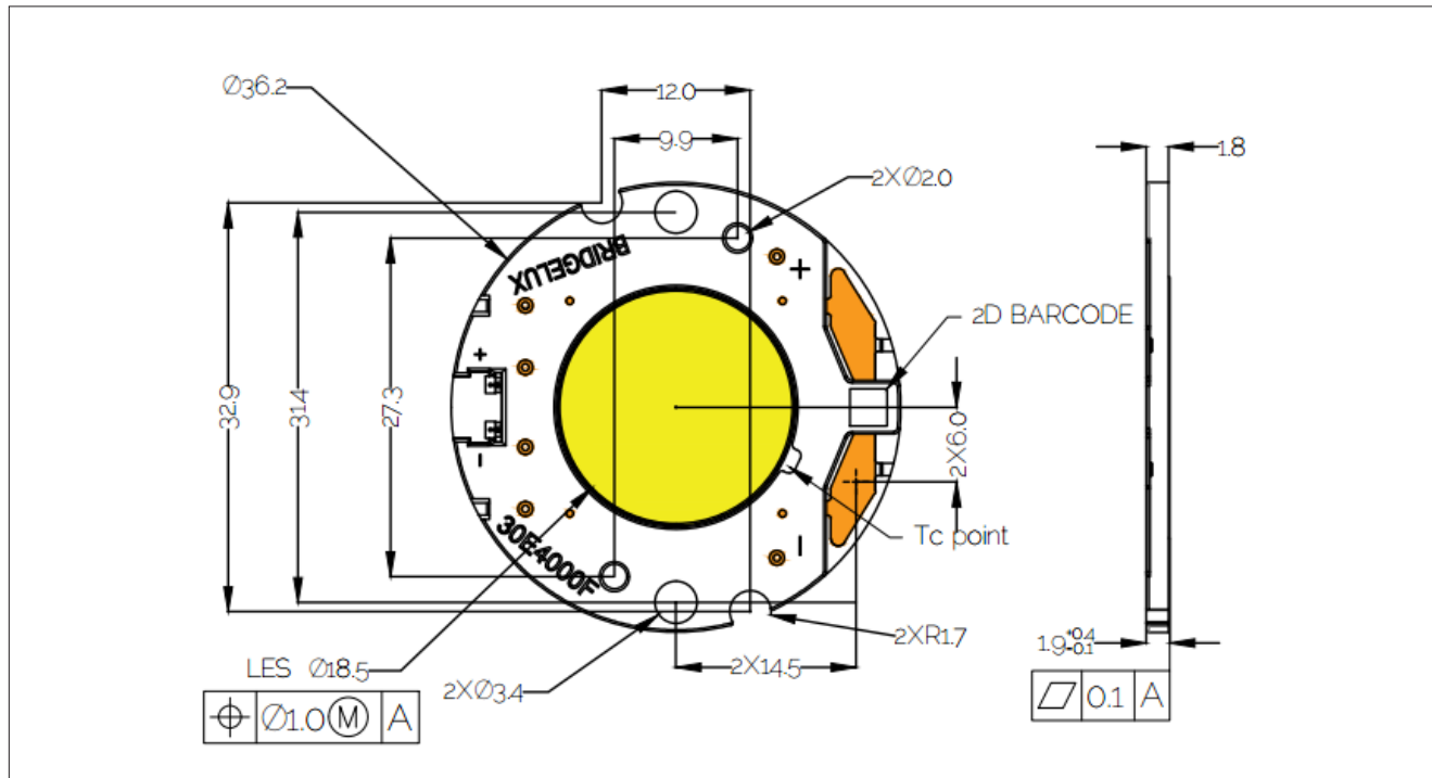
Figure 17: Drawing for Vero18 LED Array
