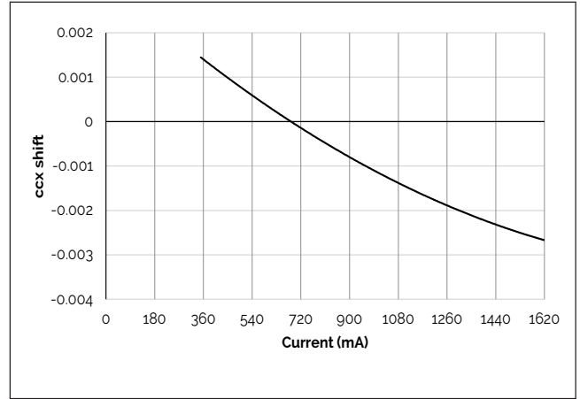
Figure 8: Vero18B Drive Current vs. ccx Shift
