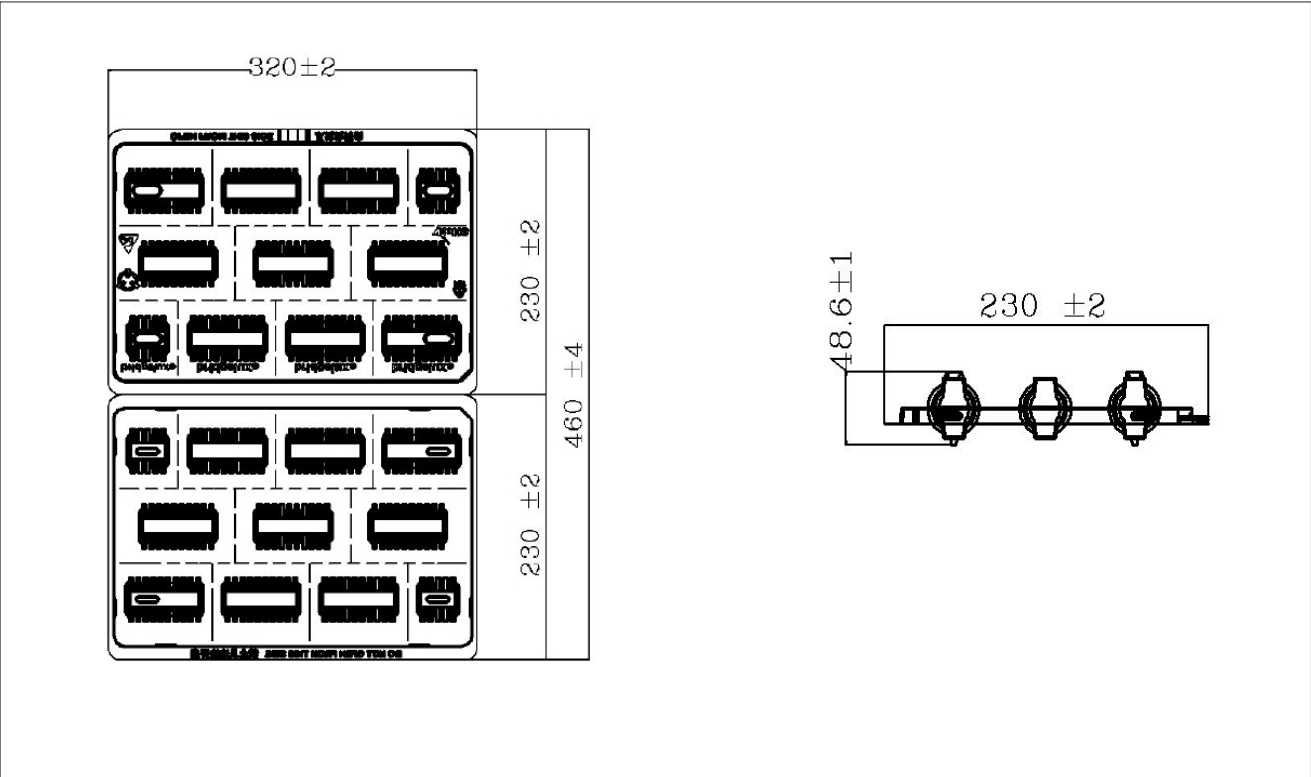
Figure 18: Drawing for Vero 18 Packaging Tray
