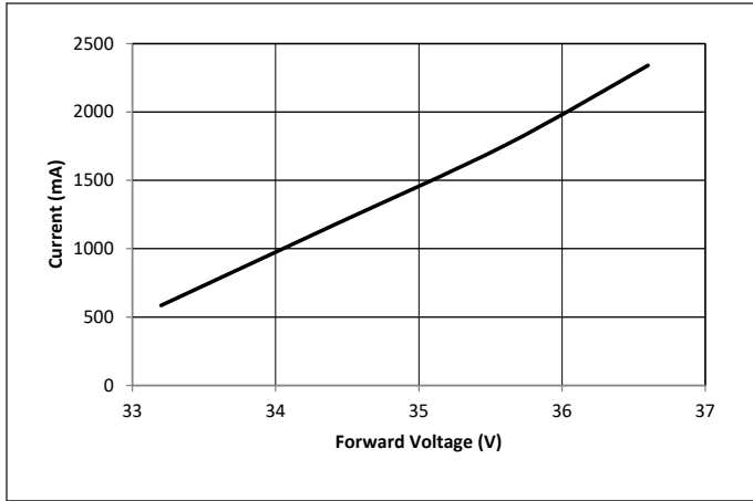
Figure 11: Vero SE 18C Drive Current vs. Voltage ( T_c=25^\circ\text{C} )
