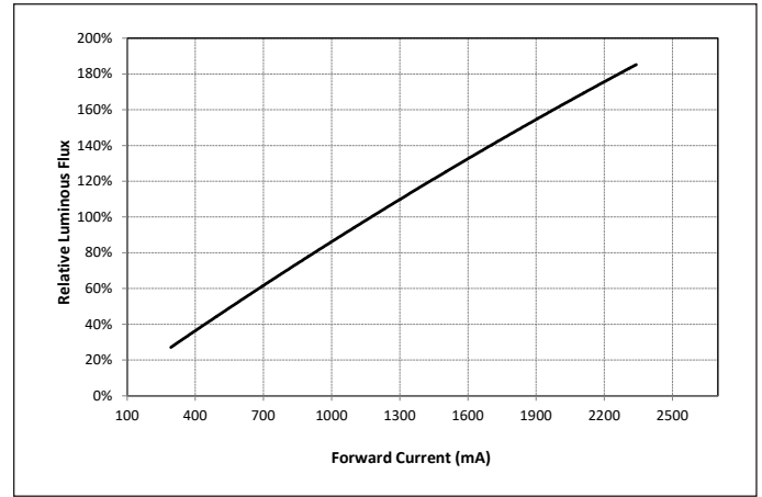
Figure 12: Vero SE 18C Typical Relative Flux vs. Current ( T_c=25^\circ\text{C} )
