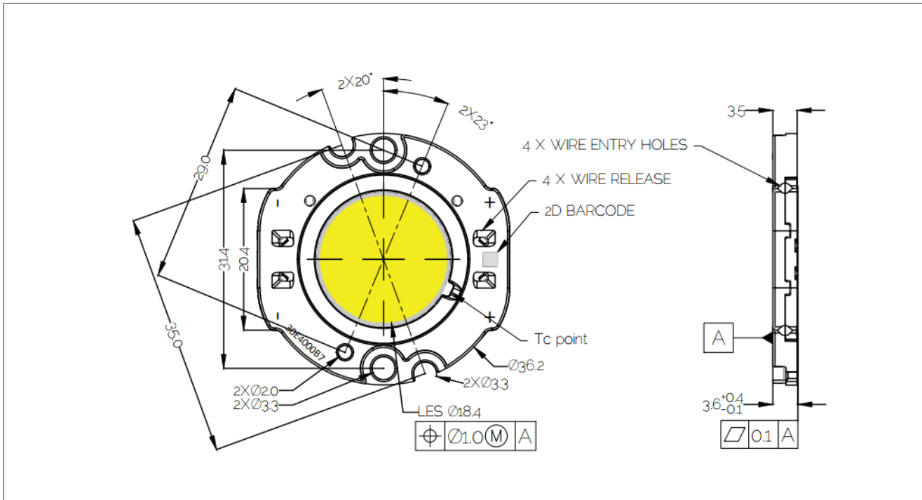
Figure 18: Drawing for Vero SE 18 LED Array
