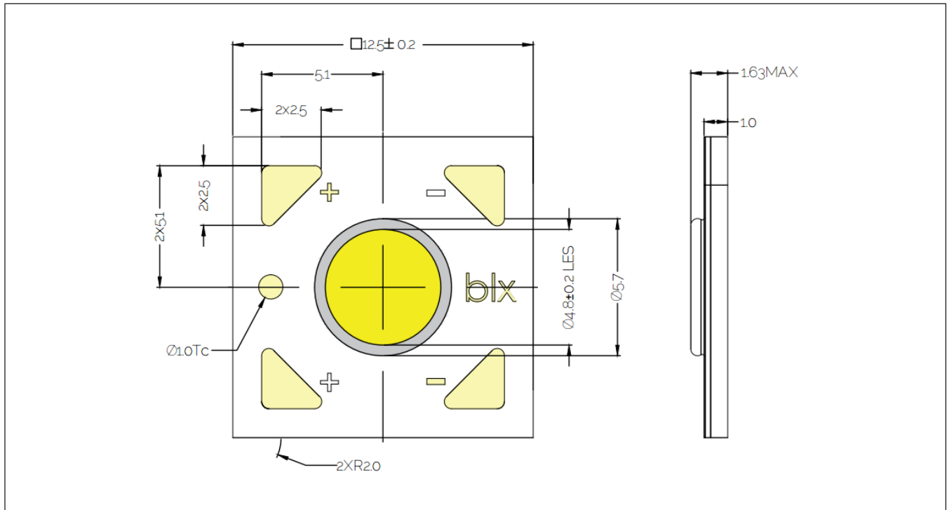
Figure 11: Drawing for V4 HD LED Array
