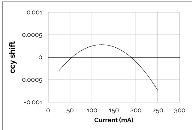
Figure 7: V4C HD Drive Current vs. ccy Shift
