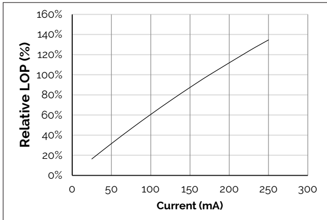
Figure 2: V4C HD Typical Relative Flux vs. Drive Current ( T_j = T_c = 25^\circ\text{C} ) 1
