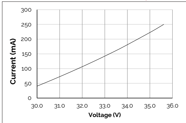
Figure 1: V4C HD Drive Current vs. Voltage ( T_j = T_c = 25^\circ\text{C} ) 1
