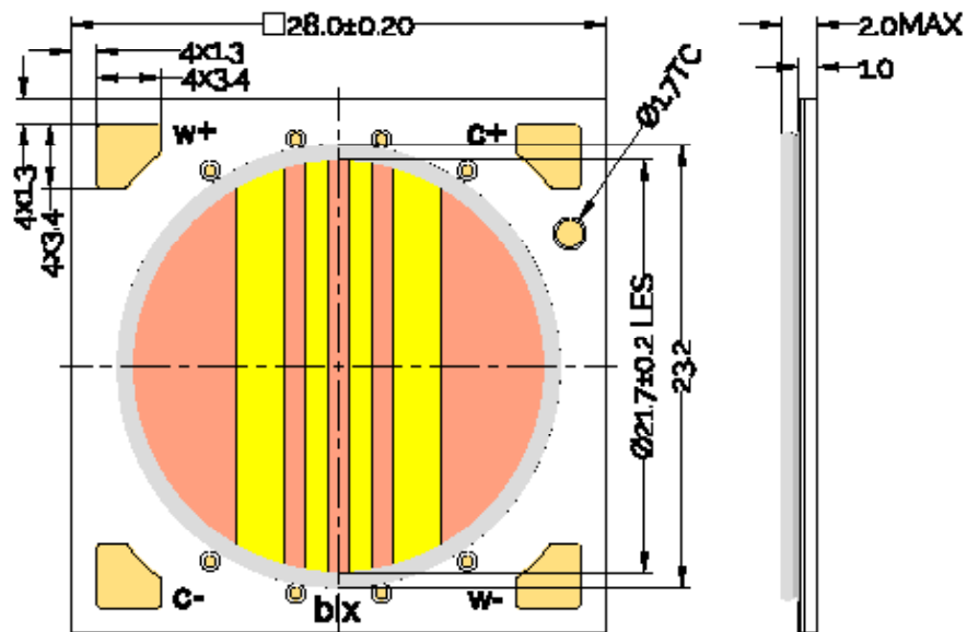
Figure 14: Drawing Specifications
