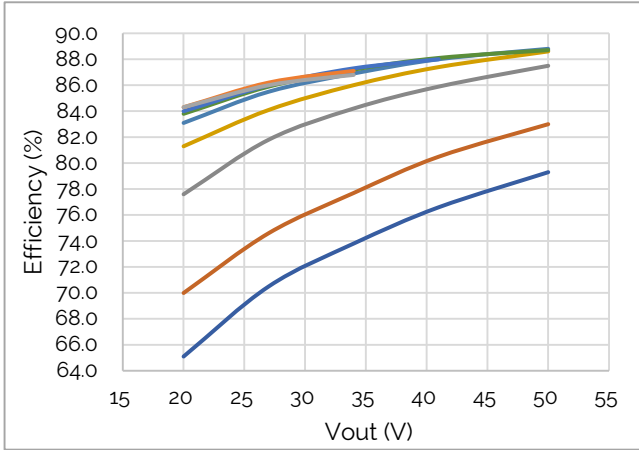
Figure 8: Efficiency @ 120VAC
