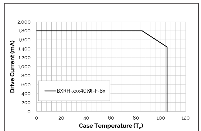
Figure 6: Derating Curve
