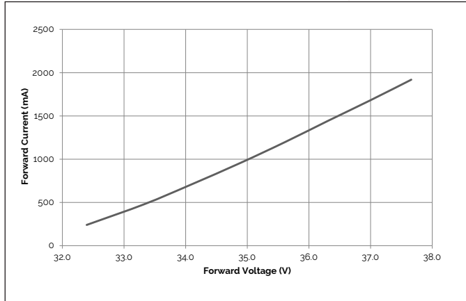
Figure 11: V15D Drive Current vs. Voltage ( T_c=25^\circ\text{C} )
