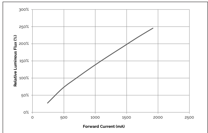
Figure 12: V15D Typical Relative Flux vs. Current ( T_c=25^\circ\text{C} )
