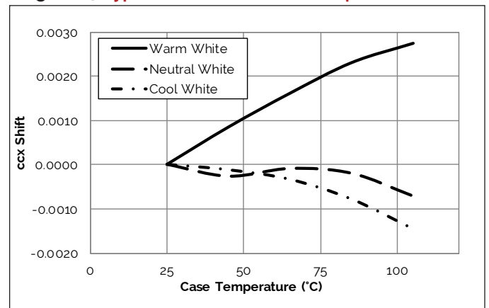
Figure 14: Typical cxx Shift vs. Case Temperature
